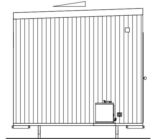
③ LEFT ELEVATION 1 : 50
